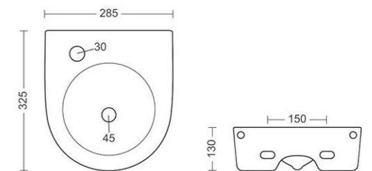
WASH BASIN L325, W285, H130MM
